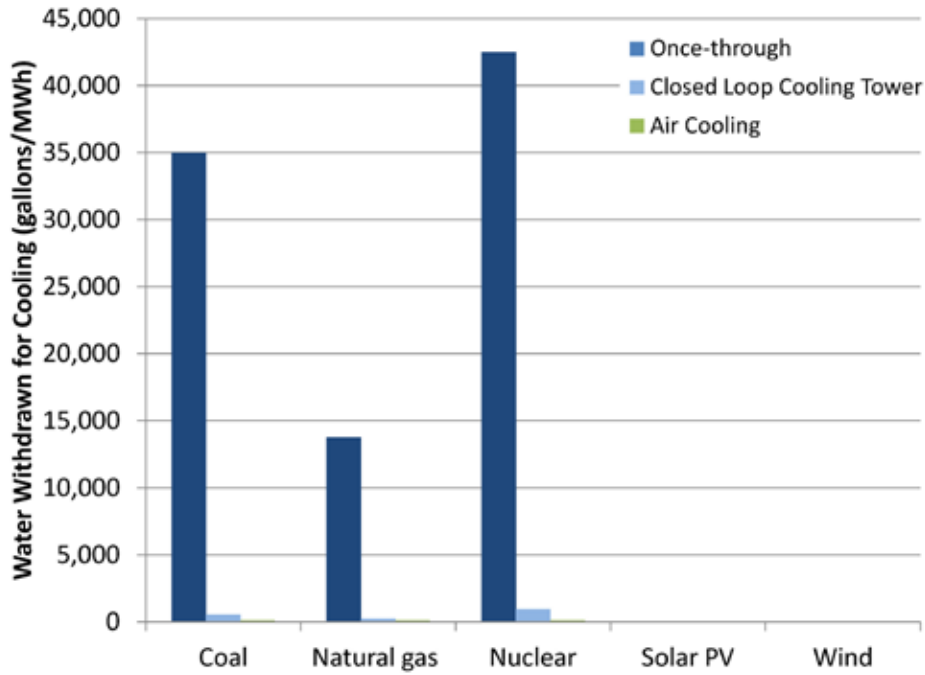
Figure 1. Comparison of Water Withdrawals by Various Cooling Technologies and Fuels 94
