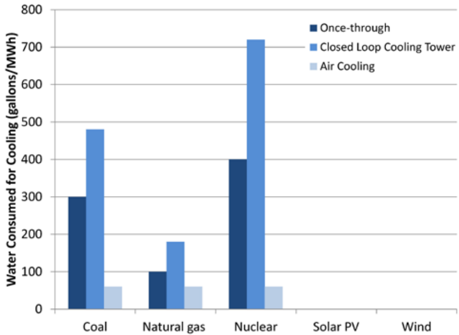
Figure 2. Comparison of Water Consumption by Various Cooling Technologies and Fuels 95
